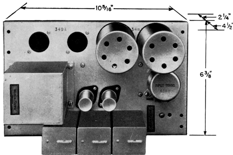
Figure 23 — 131A Monitor Amplifier.
